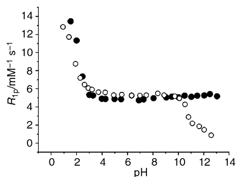
Fig. 2 pH Dependence of the longitudinal proton relaxivity of Gd·1 (open circles) and [Gd(egta)] − (filled circles) at 20 MHz and 25 °C.
