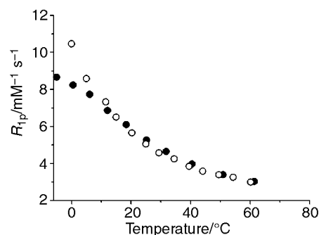
Fig. 3 Temperature dependence of the longitudinal proton relaxivity of Gd·3 (filled circles) and [Gd(egta)] − (open circles) at 20 MHz and pH 7.2.
