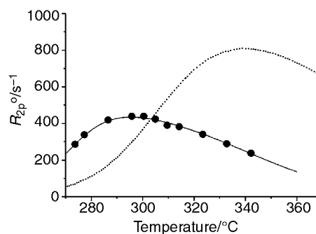
Fig. 4 Temperature dependence of the 17 O NMR transverse relaxation rate for Gd·3 (●) and calculated profile of Gd(dtpa-bma) (dotted line; parameters taken from ref. 3) for 0.055 mol L −1 aqueous solutions at 12 MHz and pH 7.2.
